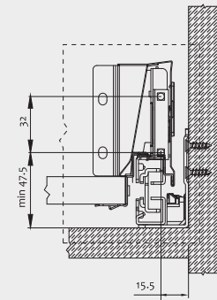
Front panel installation dimensions Front connector panel installation dimensions
