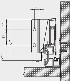
Backplane installation dimensions Back panel installation dimensions
